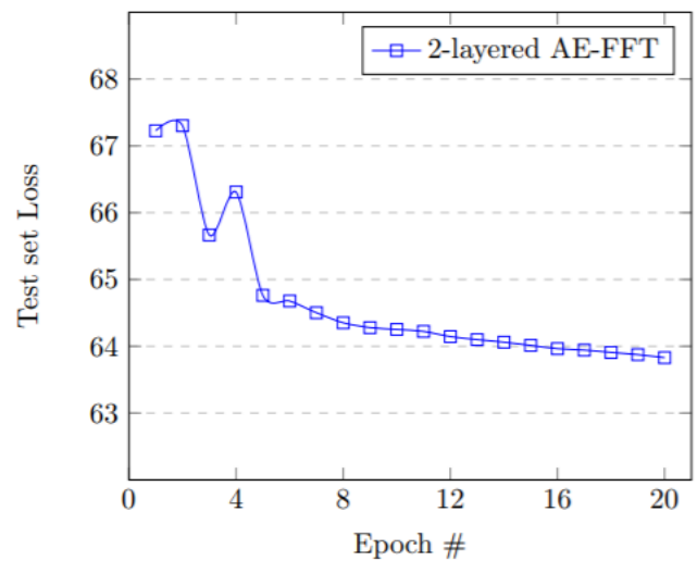
Figure 2: Test-set Loss for 2-layered AE-FFT
