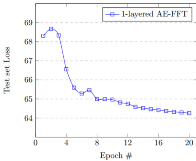
Figure 1: Test-set Loss for 1-layered AE-FFT
